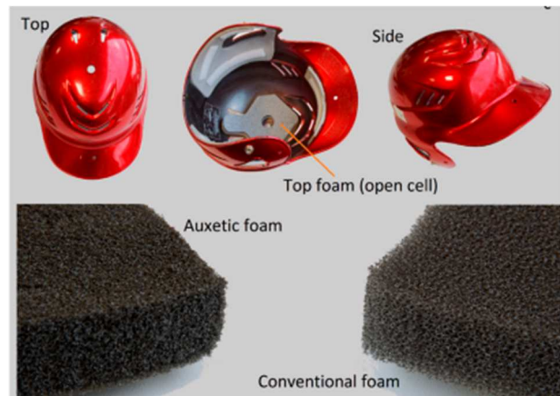
Figure 14 Application of auxetic foam in sports helmet [27]
