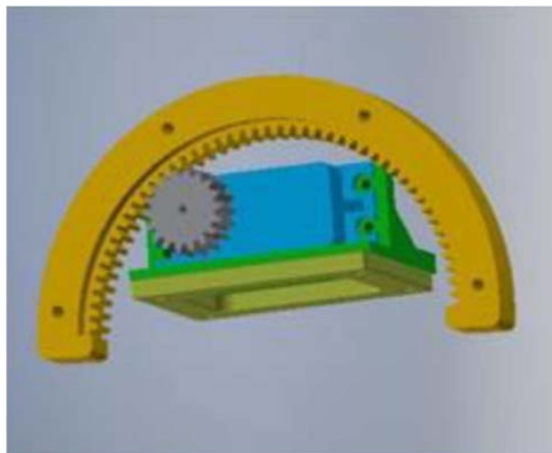
Figure 13 Transmission of the upper joint [1]
